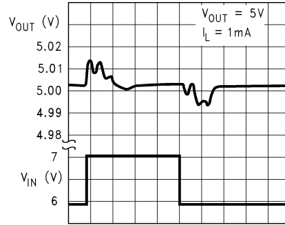
20 \mu\text{s}/\text{div} → DS012078-22
