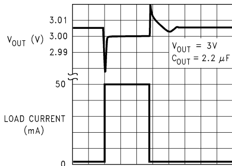
10 \mu\text{s}/\text{div} → DS012078-41
