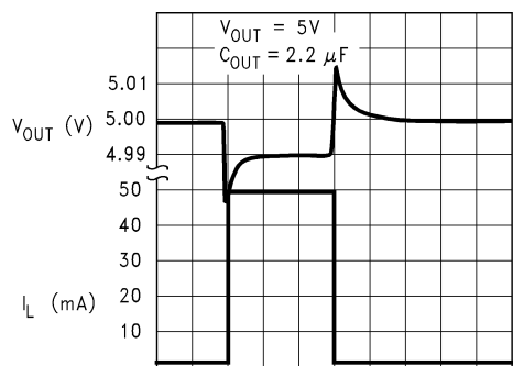
10 \mu\text{s}/\text{div} → DS012078-23
