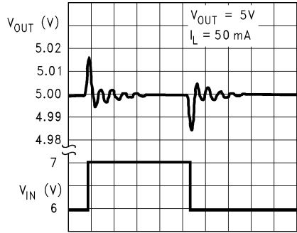
20 \mu\text{s}/\text{div} → DS012078-21
