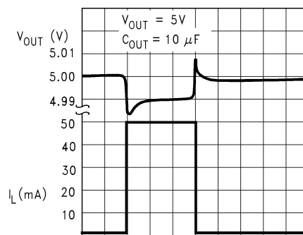
10 \mu\text{s}/\text{div} → DS012078-24
