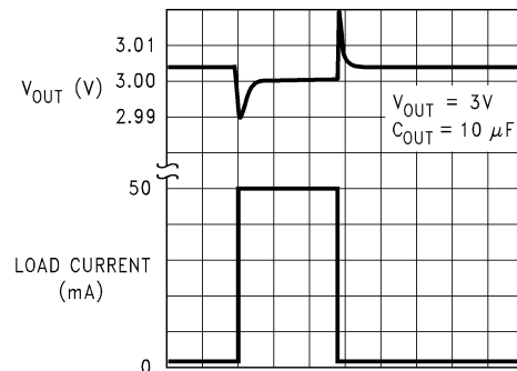
10 \mu\text{s}/\text{div} → DS012078-42
