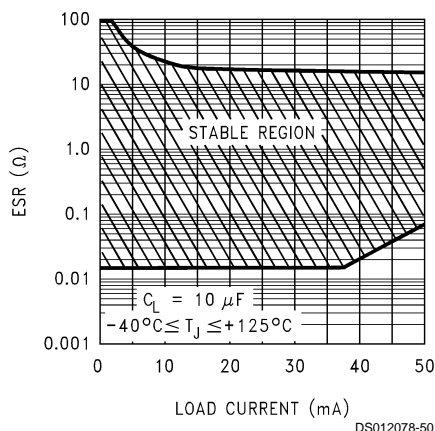
FIGURE 3. 10 µF ESR Range
